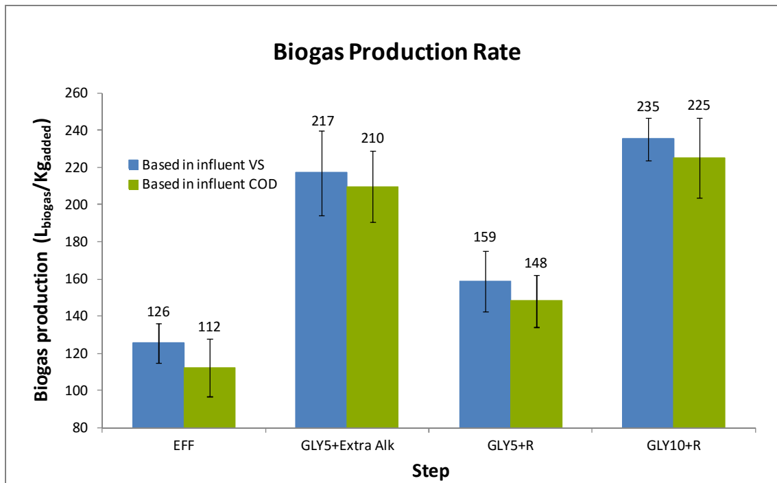
Figure 35. Biogas production rates determined in the AcD process.
