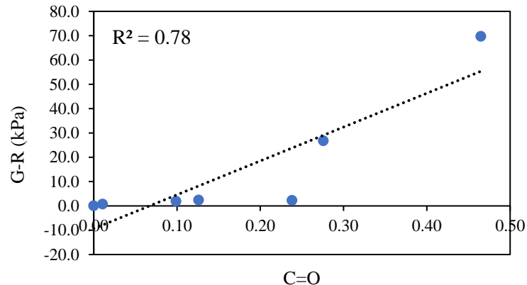
Figure 146. Carbonyl Area from Approach 2 and Glover-Rowe parameter for neat and modified blends with Binder 1 - Unaged
