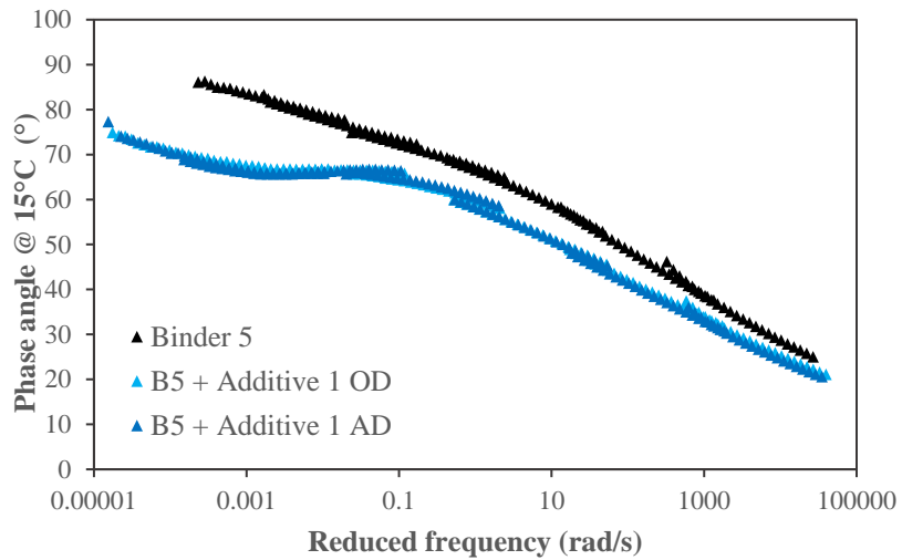
Figure 195. Phase angle master curves for Additive 1 – Binder 5 Unaged
