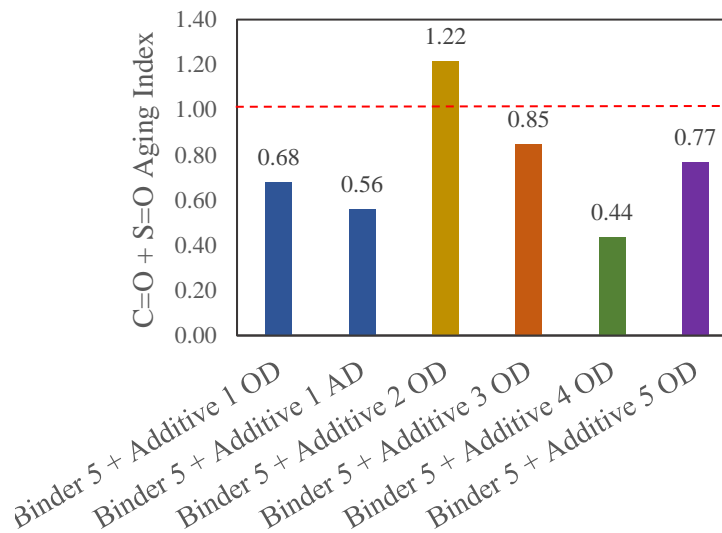
Figure 140. C=O + S=O Aging indices for Binder 5 – Approach 2
