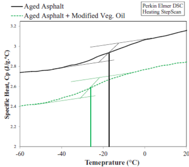
Figure 25. Glass transition temperature from heat capacity plots, for aged and rejuvenated binders (Hassan A. Tabatabaee & Kurth, 2017)
