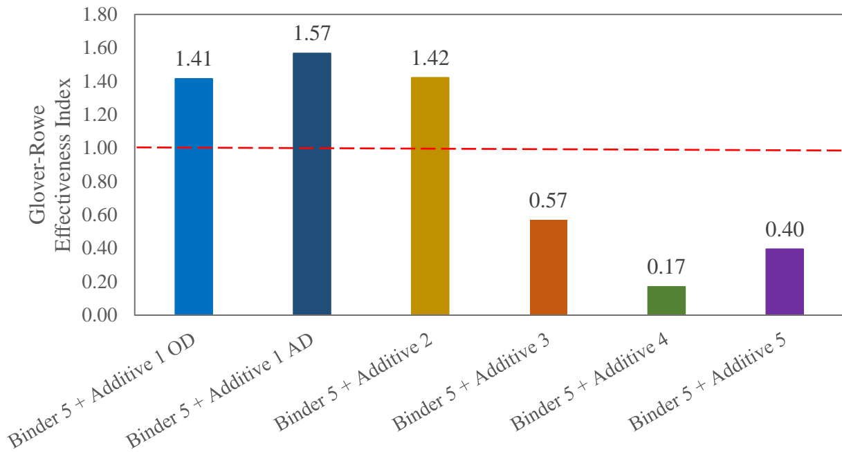
Figure 111. Glover-Rowe Effectiveness Index For Binder 5
