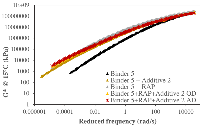
Figure 199. Complex modulus master curves for Additive 2 – Binder 5 Unaged
