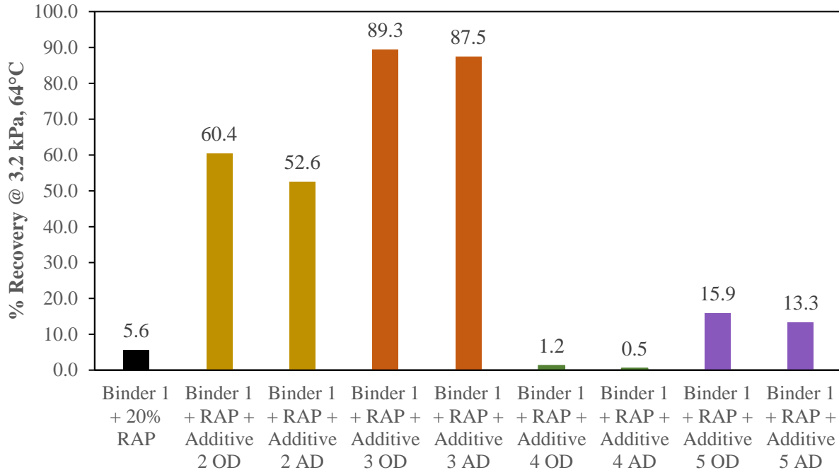
Figure 83. Elastic Recovery at 3.2 kPa - Binder 1 with RAP
